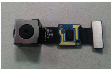
8M Camera Module (GH96-05812A)
